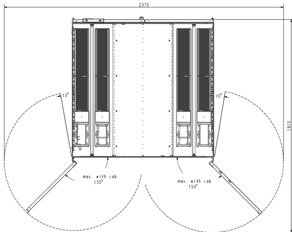
TOP-DOWN VIEW
