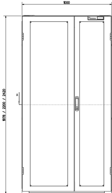
FRONT VIEW
