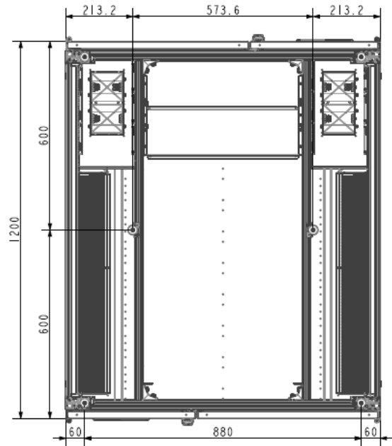
BOTTOM VIEW
