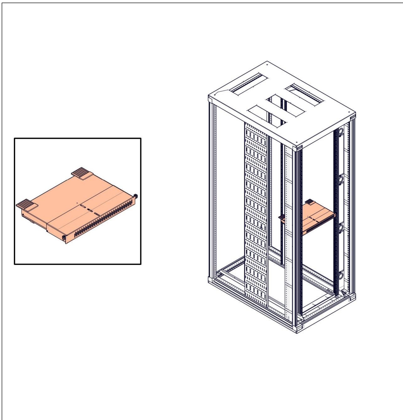
Airflow duct
