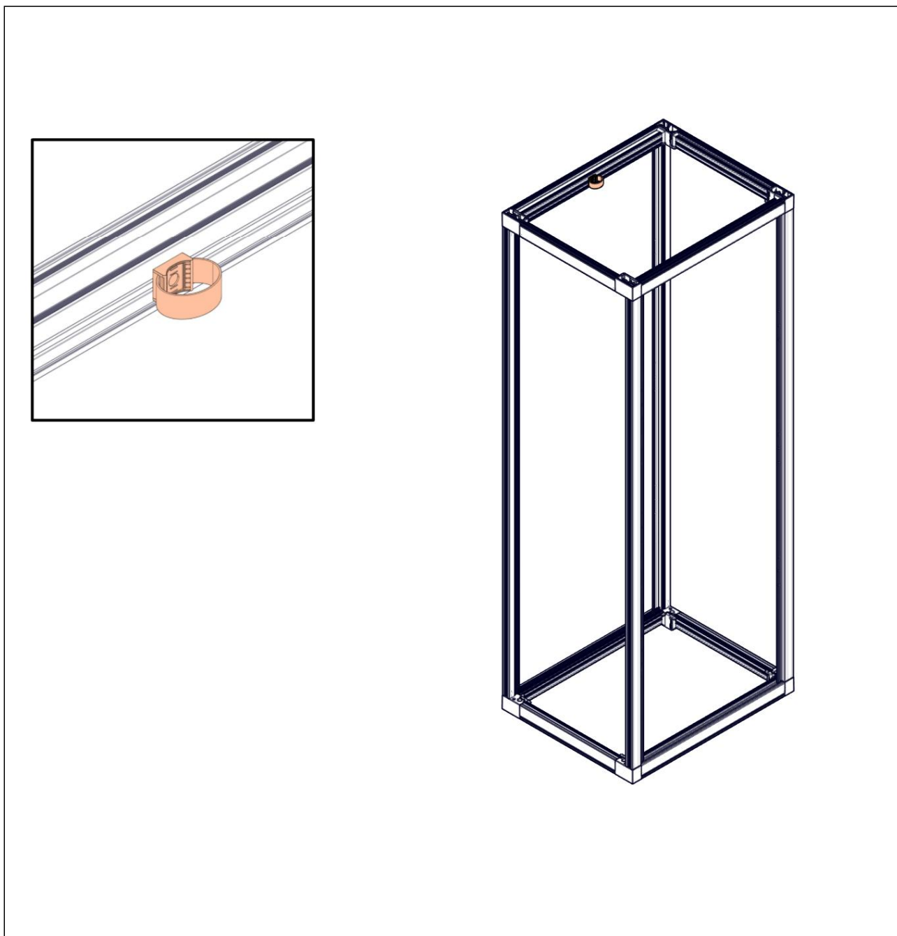
Pull relief bracket on frame
