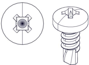
ST4.2 x 13 (SR-1)
