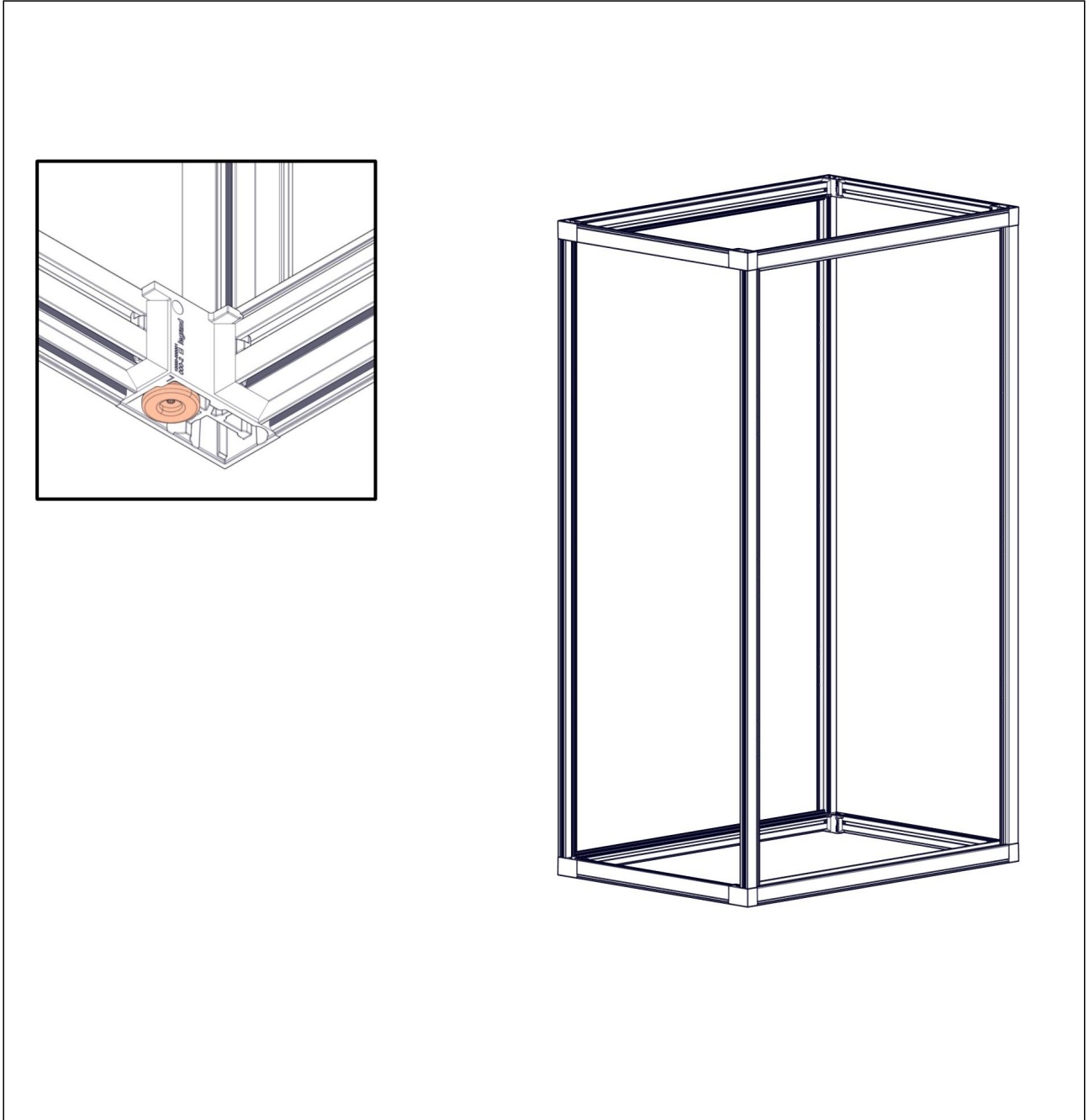
Cabinet Levelling feet
